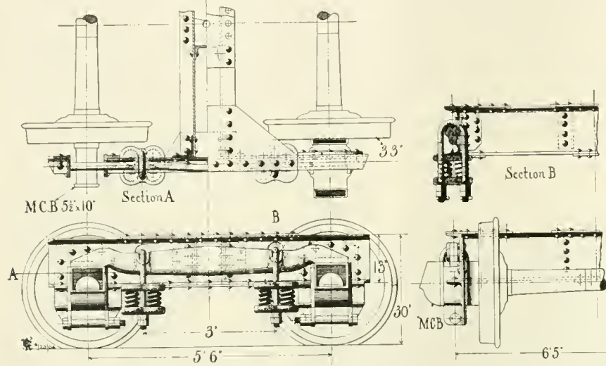
NEW DESIGN OF TENDER TRUCK.
